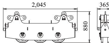
Upper Spreader (for Crane) Weight: 475 kg
